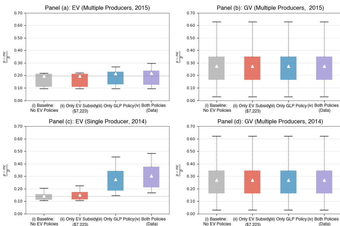
Figure 6: Markups Distribution
